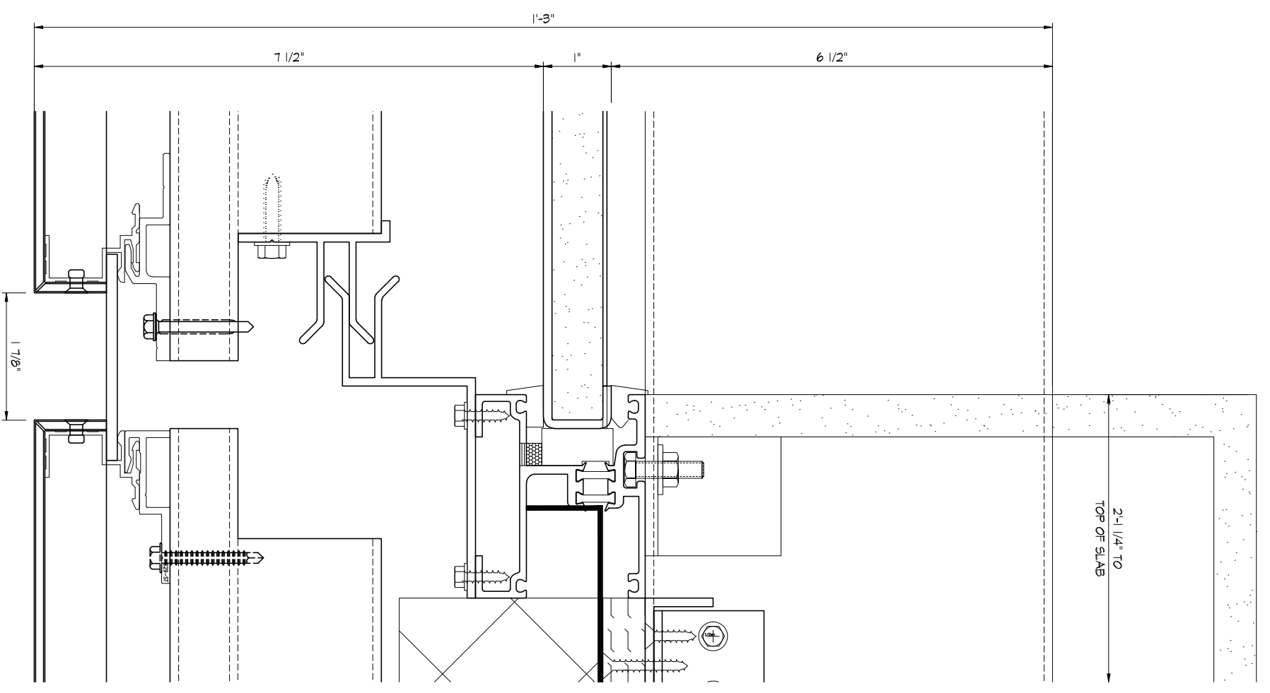
1 SILL DETAIL @ COLUMN DETAIL (EW-1a) 5.02 SCALE: FULL REF: N/A
