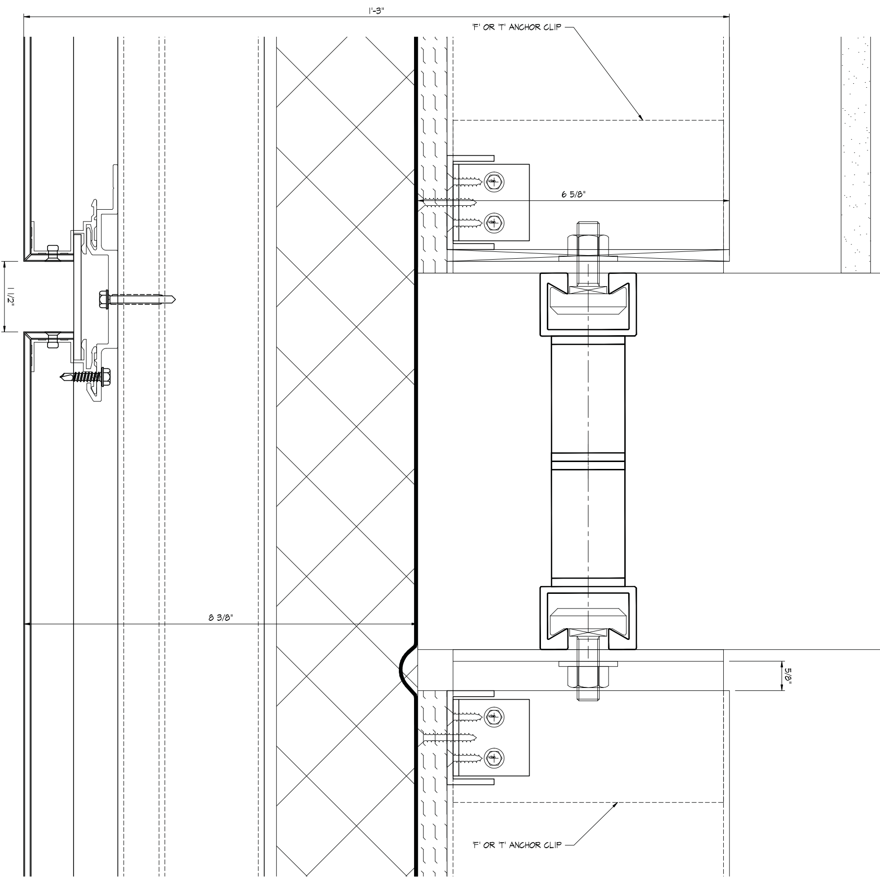
2 ANCHOR DETAIL @ WINDOW WALL (EW-1a) 5.02 SCALE: FULL REF: N/A
