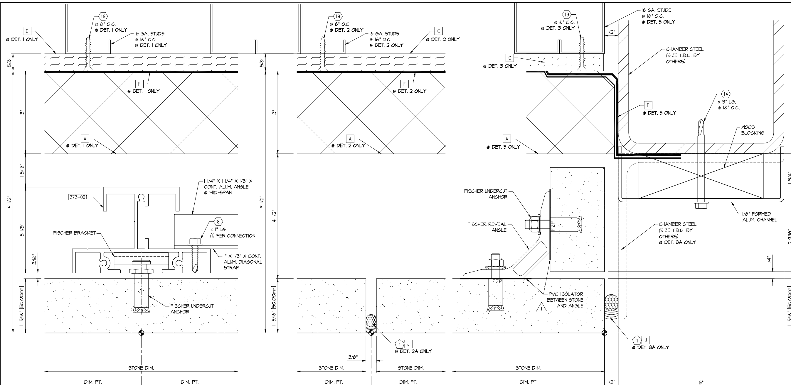
1 TYPICAL STONE MULLION D6 SCALE: FULL REF: N/A
